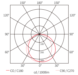
FNN1 30K-C90-1M 55lm/W 423.4lm
