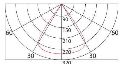
Polar Luminous Intensity Distribution
